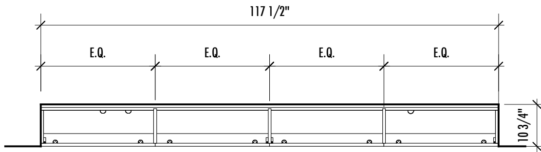
505 A.V. UNIT PLAN SCALE 1/2"=1'-0"
