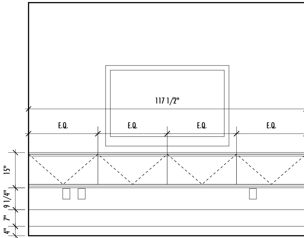
505 A.V. UNIT ELEVATION SCALE 1/2"=1'-0"
